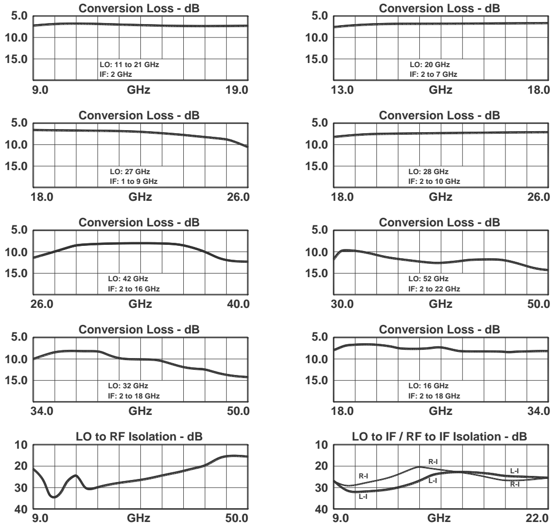
Typical Performance
