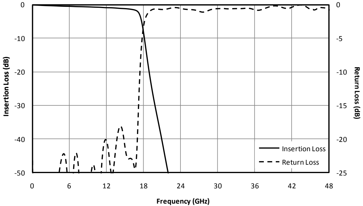
Fig. 1. Magnitude response for a typical FLP-1740.
