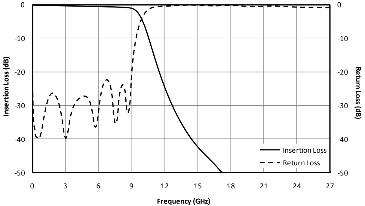
Fig. 1. Magnitude response for a typical FLP-0960.
