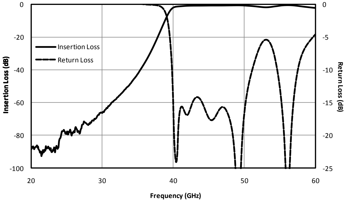
Fig. Magnitude response for a typical FH-4000 Filter.
