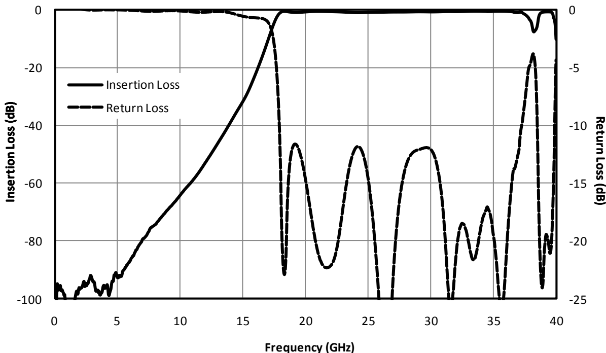
Fig. Magnitude response for a typical FH-1800 Filter.
