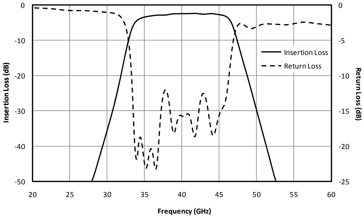
Fig. 1. Magnitude response for a typical FB-4000.
