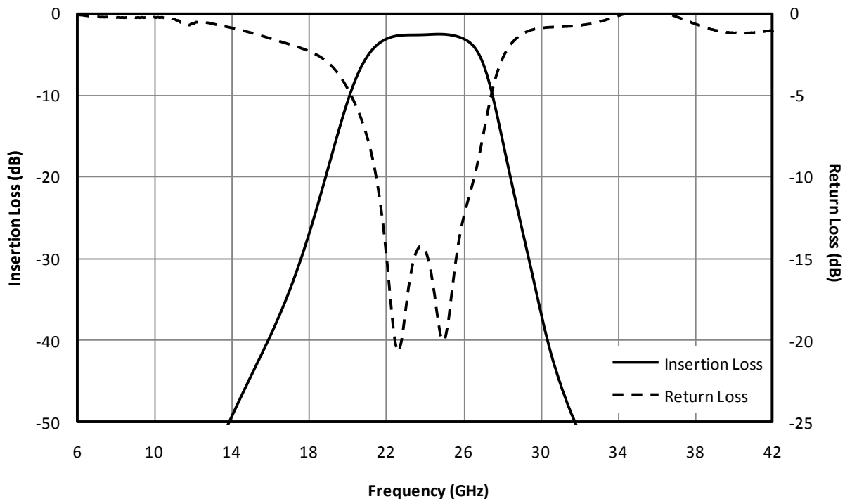
Fig. 1. Magnitude response for a typical FB-2400.
