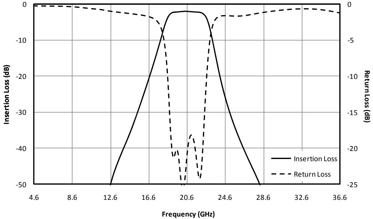
Fig. 1. Magnitude response for a typical FB-2060.
