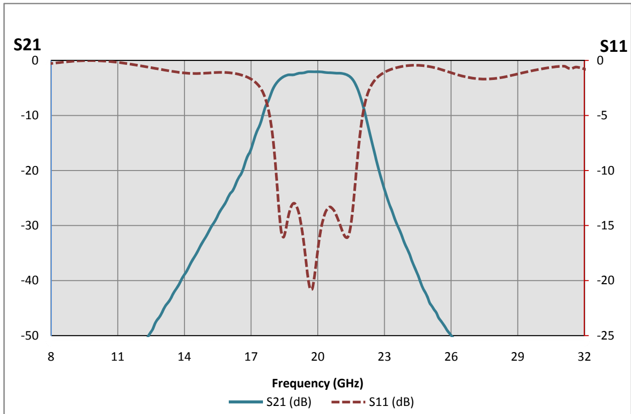
Magnitude response for a typical 20 GHz Band Pass Filter.
