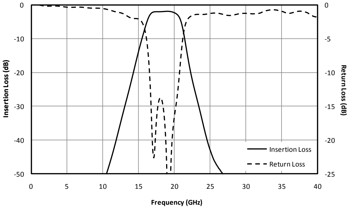
Fig. 1. Magnitude response for a typical FB-1840.
