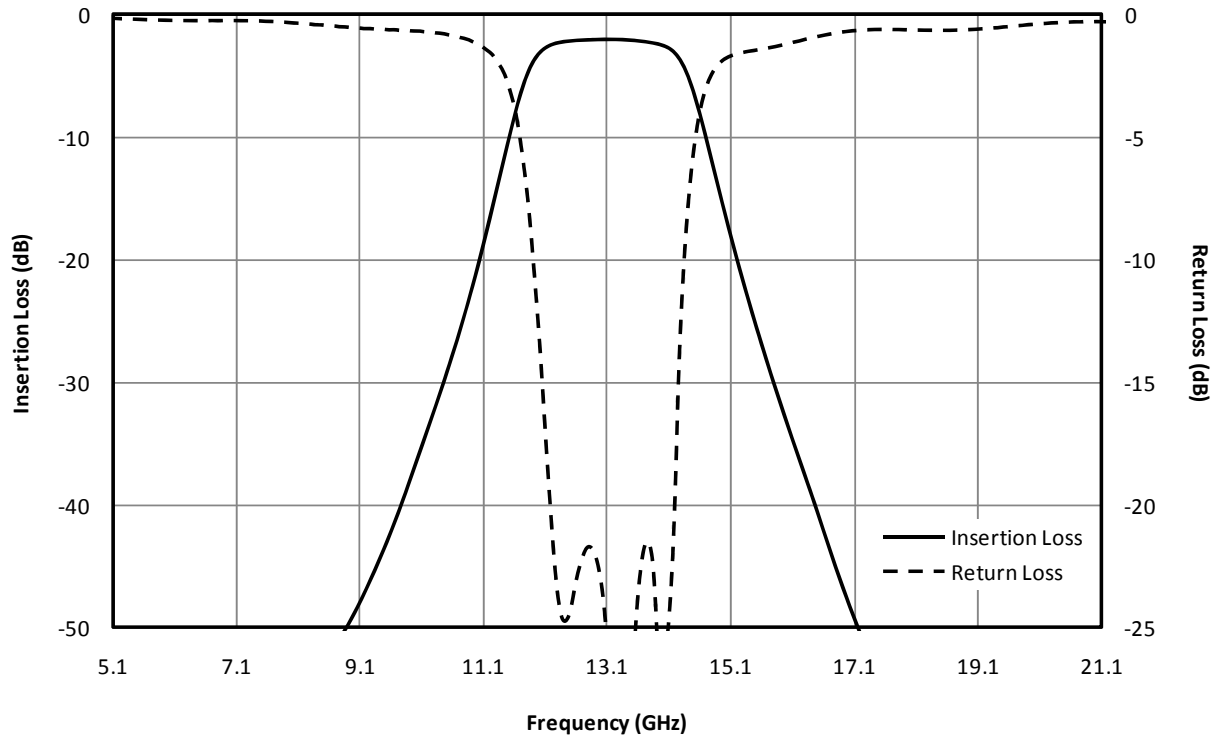
Fig. 1. Magnitude response for a typical FB-1310.
