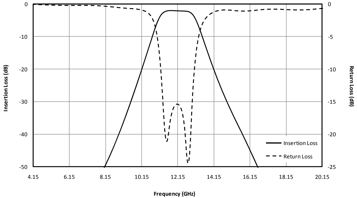
Fig. 1. Magnitude response for a typical FB-1215.
