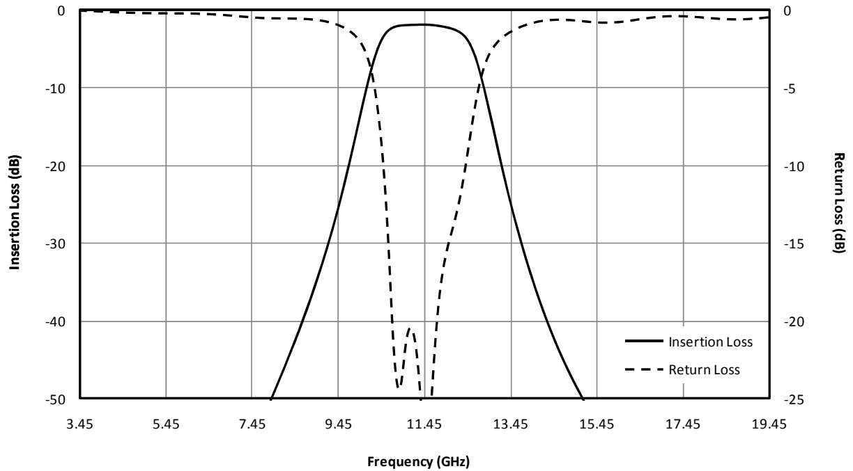
Fig. 1. Magnitude response for a typical FB-1145.
