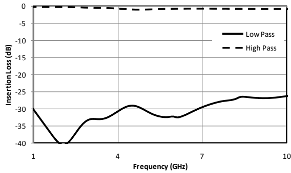
Fig. 6. Insertion loss.
