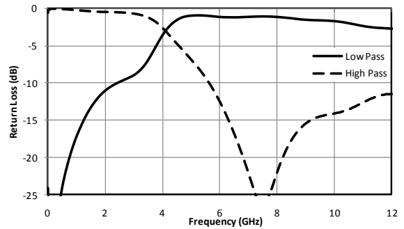
Fig. 3. Return loss.
