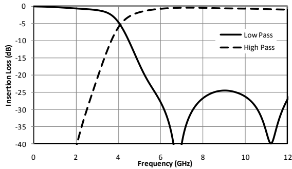
Fig. 2. Insertion loss.
